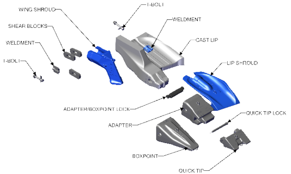
FIGURE 1. Cast lip and G.E.T. labels
