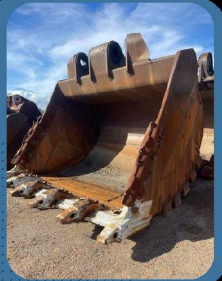
Hitachi EX3600-6
