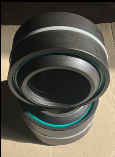
793F RAX LINK BEARING (NEW) PN 2993203, MSPN-0001953
