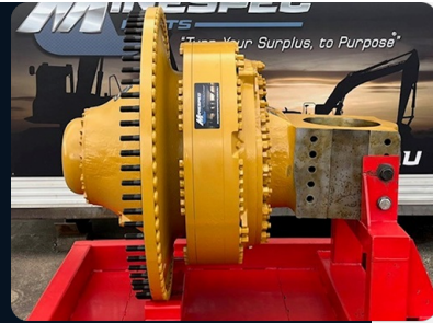
793D Front Wheel Group PN 2527174
